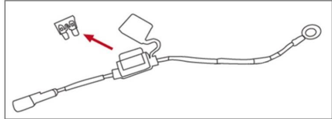
Open fuse holder cap and remove fuse
