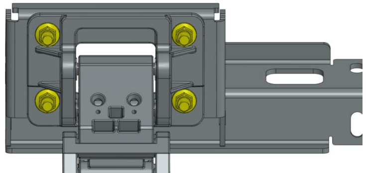
Tighten the M8 Flanged Nylon Lock Nuts all the way until tight.
