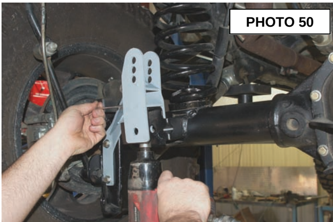
Insert bolt from front side
