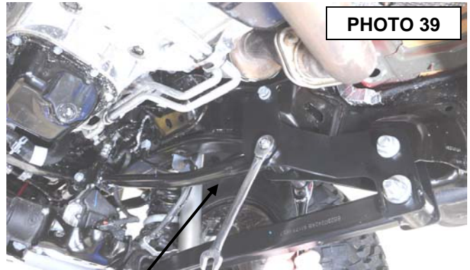
Tighten upper control arm.
