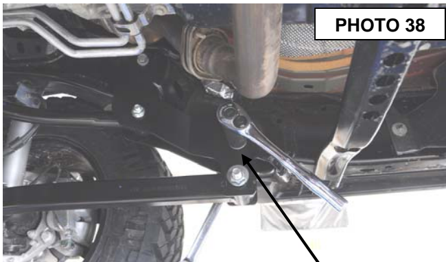
Tighten the lower drop hardware.
