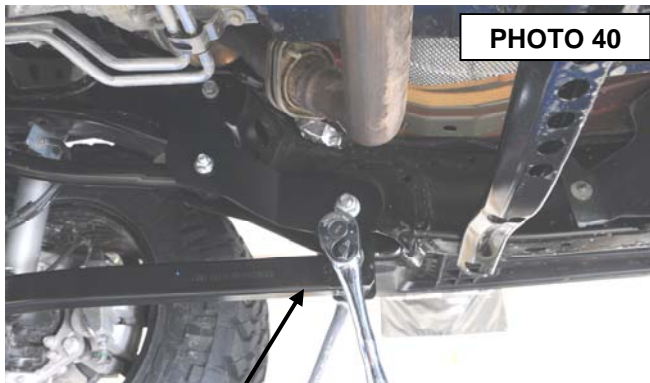
Tighten lower control arm.
