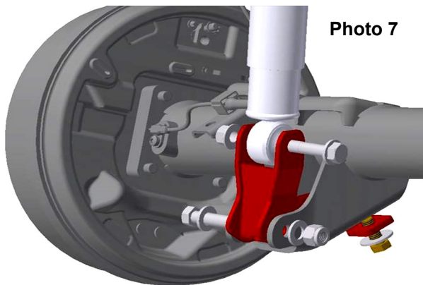
Install Magneride shock relocation brackets.
