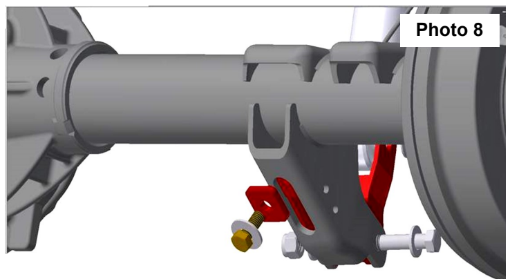
Install Magneride shock relocation brackets.
