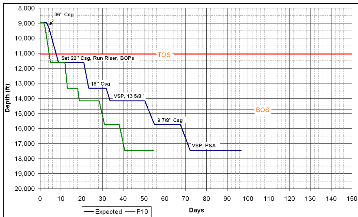
Figure 3-3 Days vs Depth Dryhole
