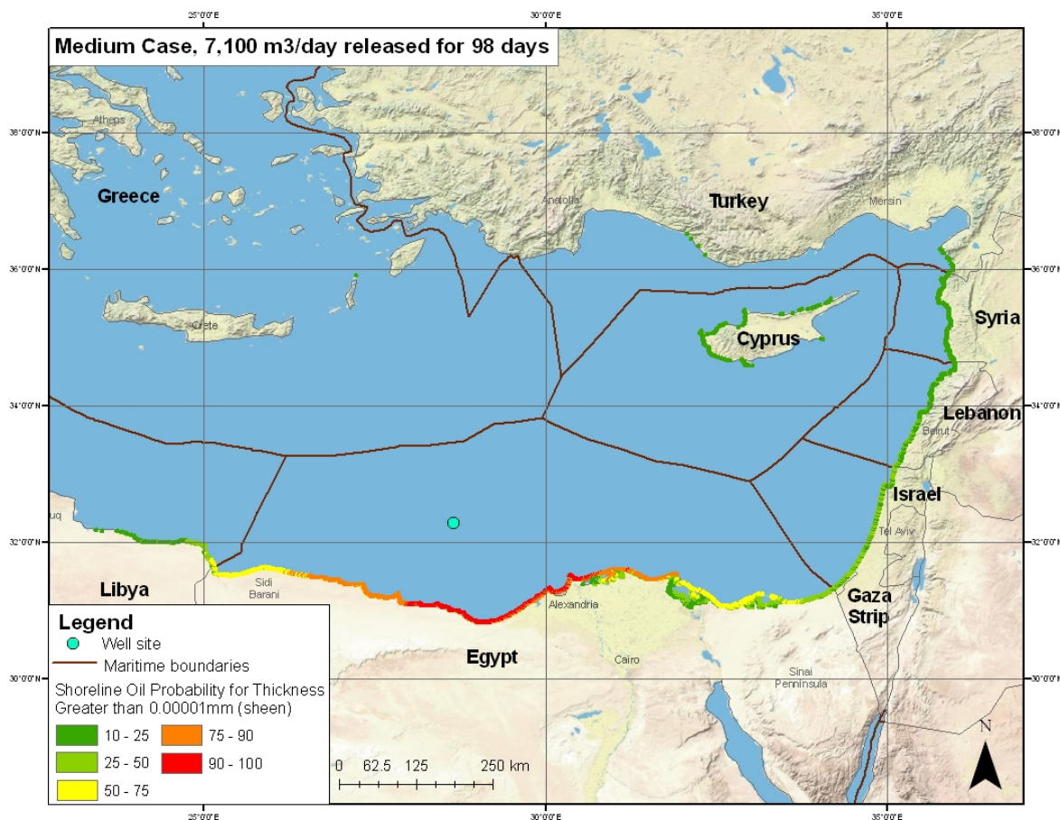
Figure 4-6 Probability Distribution of Oil on Shorelines
