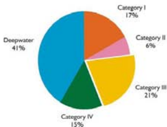
Graph - 2.1 : Category-wise Distribution of Sedimentary basins in India
