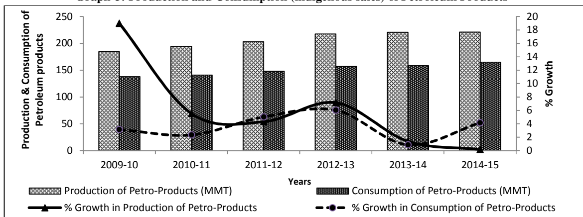
Graph-3: Production and Consumption (indigenous sales) of Petroleum Products
