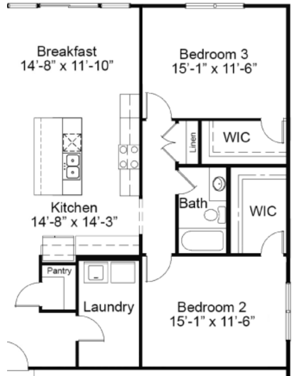
OPTIONAL EXPANDED BEDROOM 3
