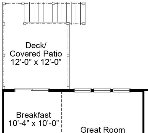
OPTIONAL DECK/COVERED PATIO
