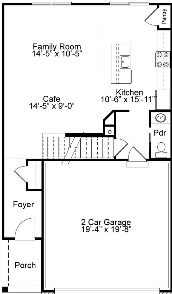
OPTIONAL FIRST FLOOR WITH LUXURY KITCHEN
