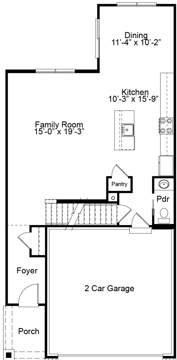
OPTIONAL DINING ROOM PLAN
