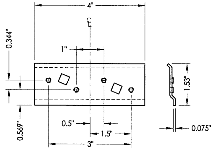
29 HINGE REINFORCEMENT
