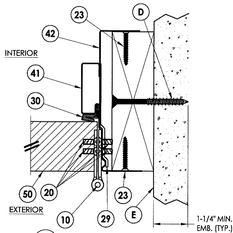
3 4 HORIZONTAL CROSS SECTION 2X wood buck
