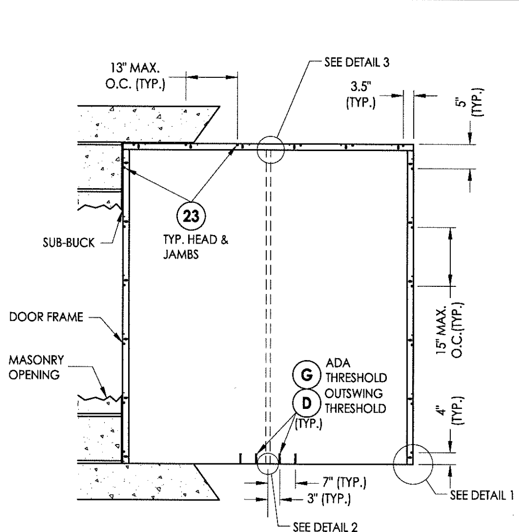
FRAME ANCHORING Masonry 2X buck construction
