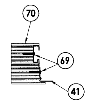
DETAIL 1 ADA Threshold
