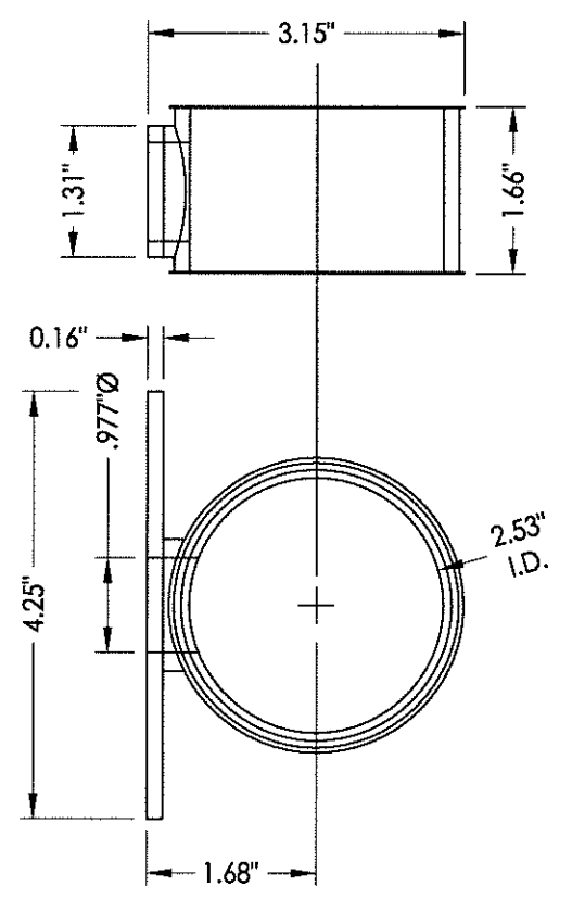
1A LOCK RING
