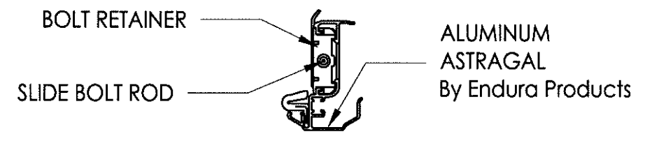
VIEW A-A Aluminum Astragal Assembly
