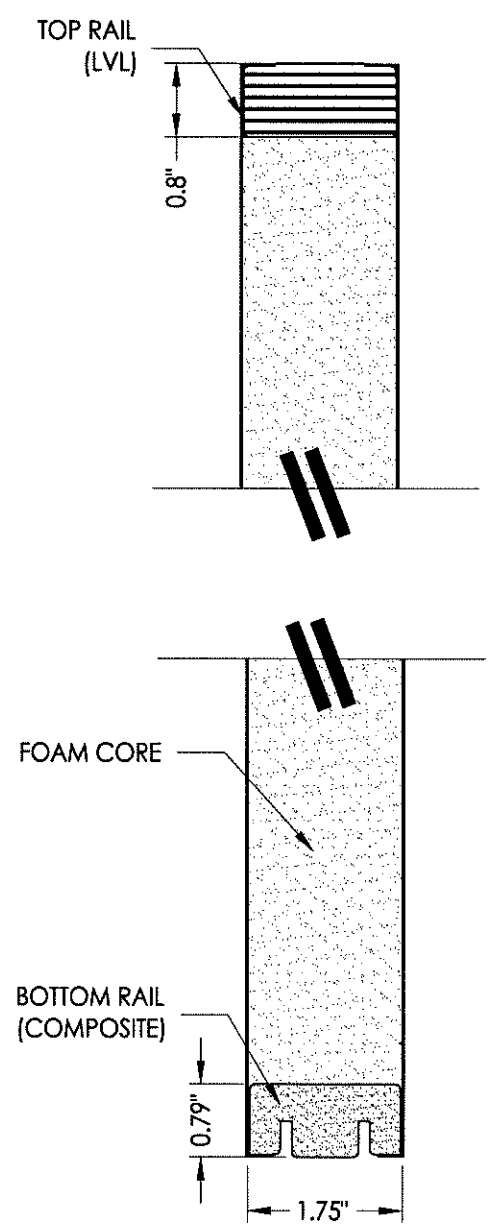
2 VERTICAL CROSS SECTION 3 Door panel
