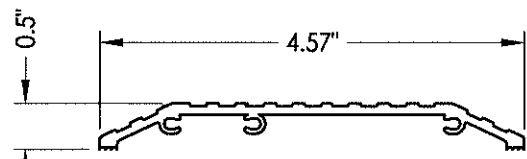
70 ADA THRESHOLD Imperial
