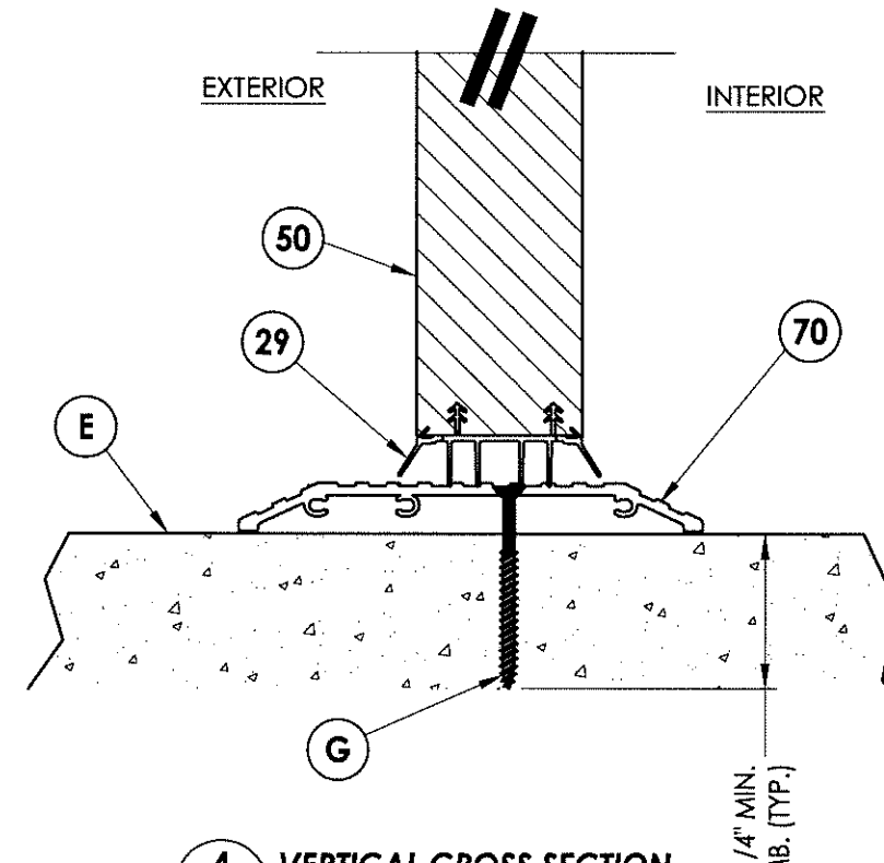
4 VERTICAL CROSS SECTION 5 Shown w/ ADA Threshold
