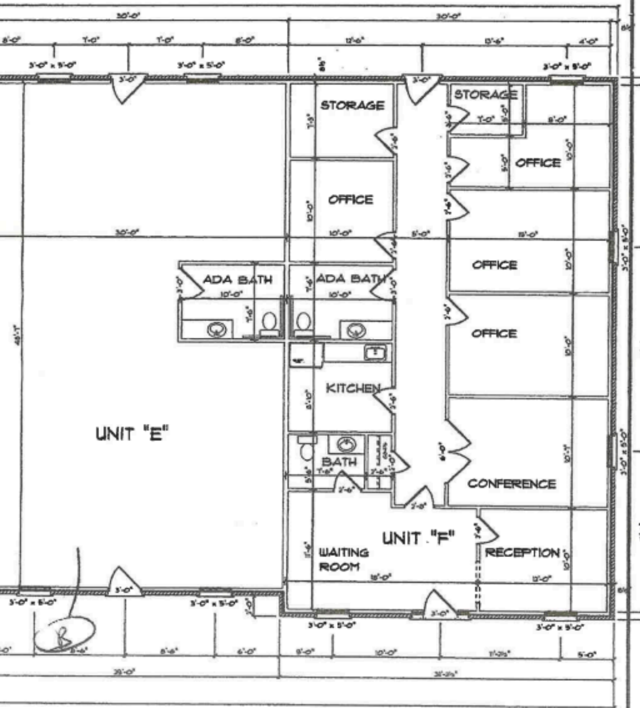
FLOOR PLAN - BUILDING #1
