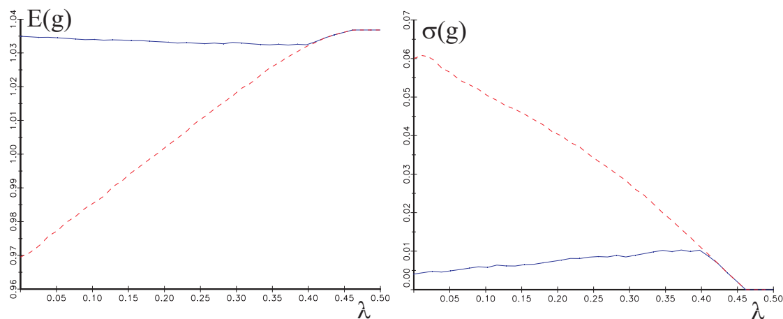
Figure 3: Mean and standard deviation of growth as \lambda varies from 0 to 0.5 where A = 1.08 , \beta = 0.96 , \pi = 0.9 and z = 0.85 . The secured-borrowing equilibrium is shown by the red (dashed) curve, and the equilibrium with secured and unsecured borrowing is blue (solid). E(g) and \sigma(g) are calculated as sample averages for a time series of 50,000 periods.
