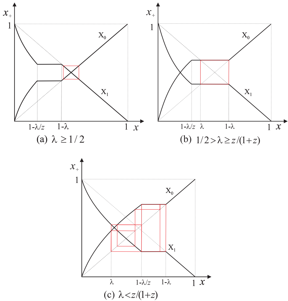
Figure 1: Asymptotic cycles with secured borrowing.
