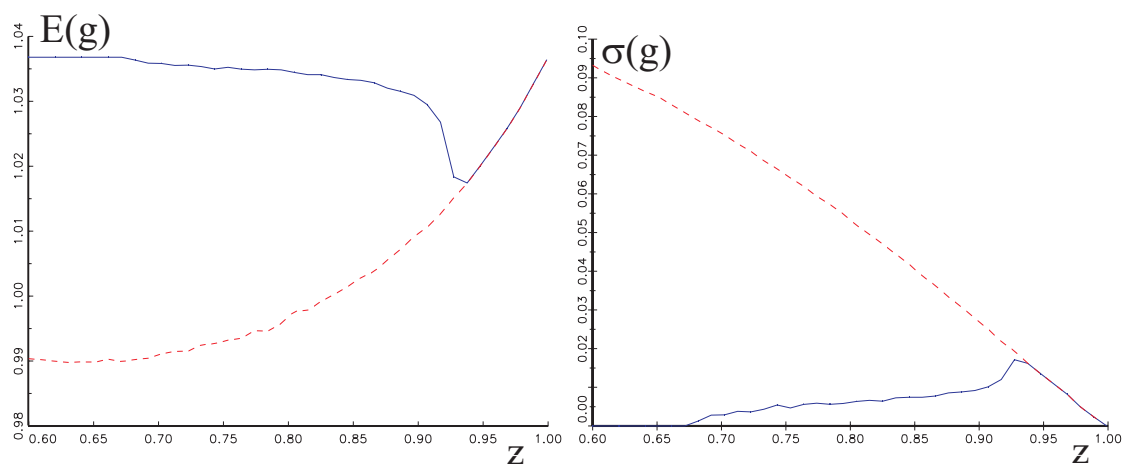
Figure 4: Mean and standard deviation of growth as z varies from 0.6 to 1 where A = 1.08 , \beta = 0.96 , \pi = 0.9 and \lambda = 0.2 . The secured-borrowing equilibrium is shown by the red (dashed) curve, and the equilibrium with secured and unsecured borrowing is blue (solid). E(g) and \sigma(g) are calculated as sample averages for a time series of 50,000 periods.
