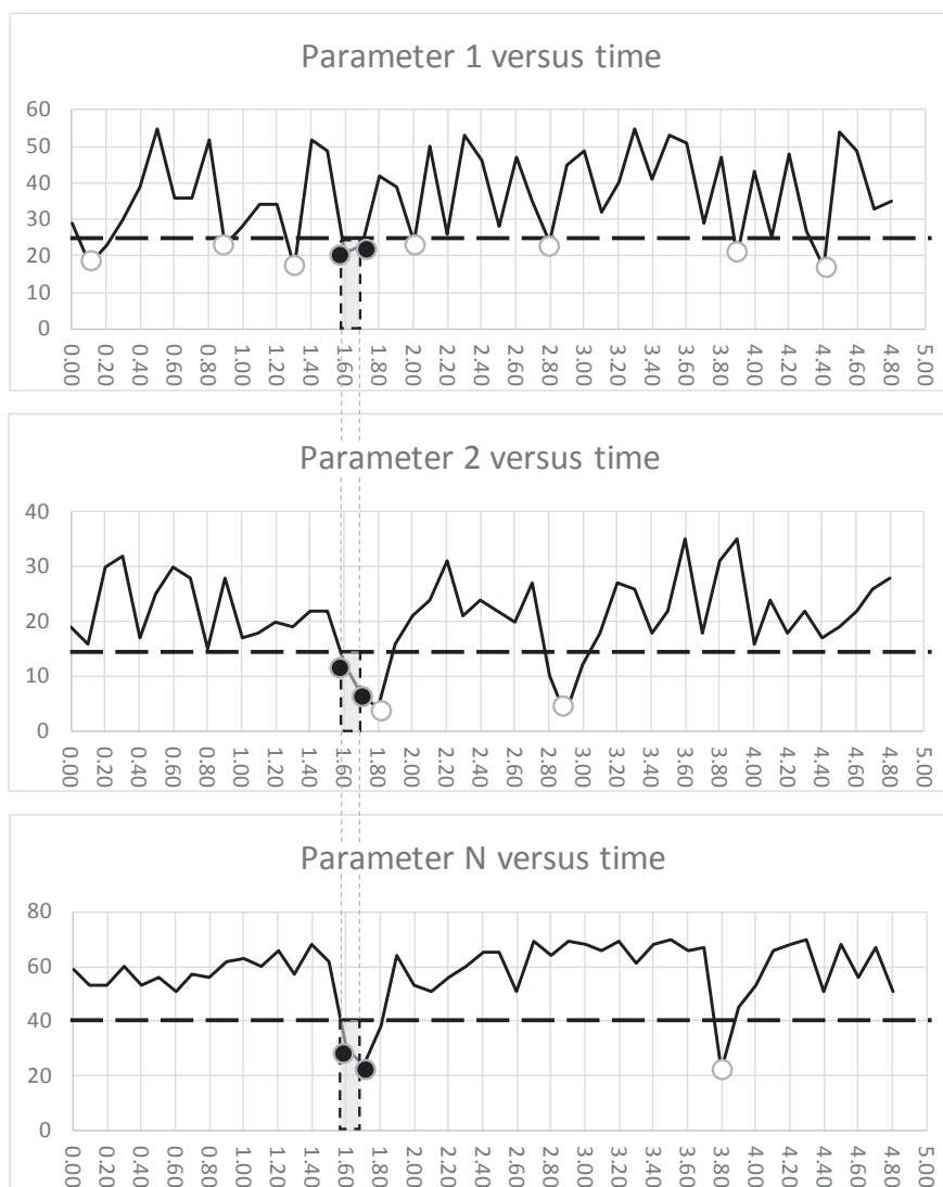
Figure 5. Multiple measurements plotted against time. Combinatorial alarm signals are issued only when the threshold criteria for all parameters are met simultaneously. The combinatorial alarm signal can have the effect of reducing the overall alarm reporting frequency due to false alarms because the potential for individual measures all meeting their threshold criteria simultaneously is hypothesized to be more likely associated with a true-positive event than false alarm signals.
