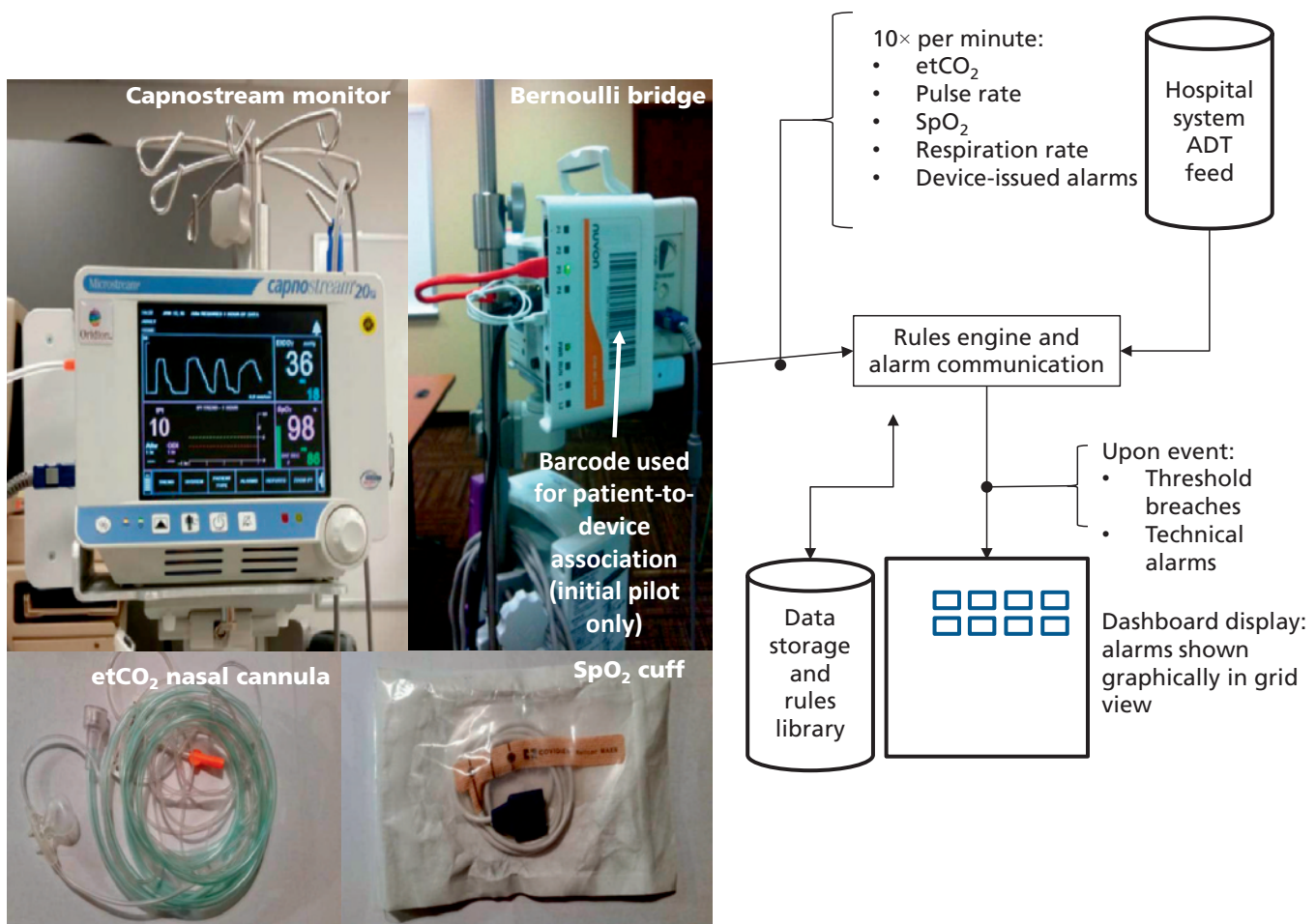
Figure 1. Capnostream 20p monitors communicated through Bernoulli IDM 3400 serial-to-ethernet bridges. Bridges would poll the monitor at the rate of 10 times per minute and communicate data wirelessly to the Bernoulli Analytics Software located within the enterprise data center. Rules were maintained within the Bernoulli data storage and rules library and recalled for application against the received data. The serial-to-ethernet bridges were outfitted with barcodes to facilitate a patient-to-device association workflow using a Gryphon barcode reader. Also shown are the data collection and alarm signal communication from the monitors to the dashboard displayed within the telemetry bunkers. Abbreviations used: ADT, admission discharge transfer; etCO 2 , end-tidal carbon dioxide; SpO 2 , peripheral capillary oxygen saturation.
