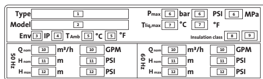
Fig. 1 Nameplate for pump
