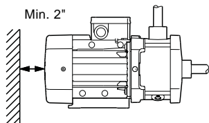
Fig. 5 Allow minimum 2" distance from motor fan to a surface
