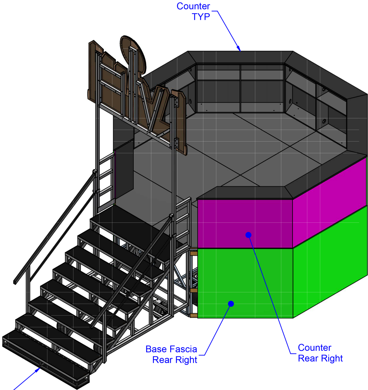
REAR ISOMETRIC
