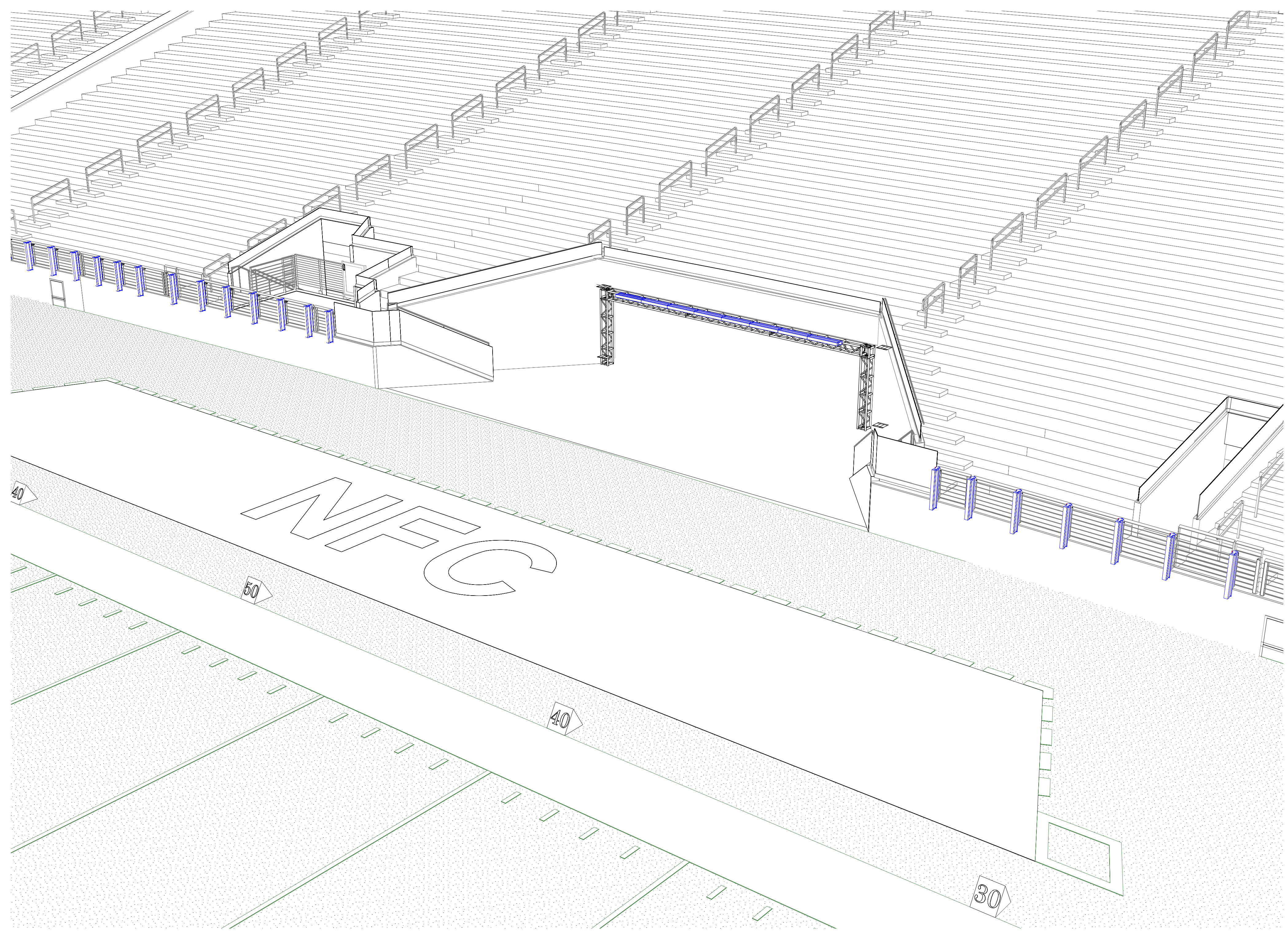
B LEVEL 100 EAST 50 YD LINE GOAL POST PERSPECTIVE Scale: 3/4" = 1'-0"
