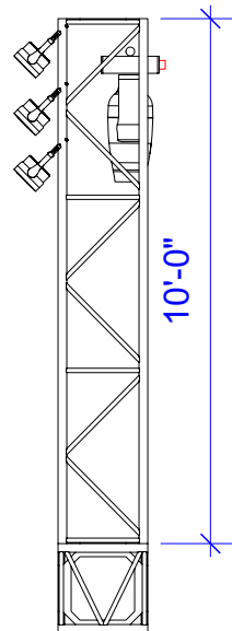
Side Elevation
