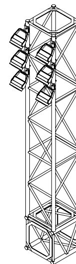
Isometric View
