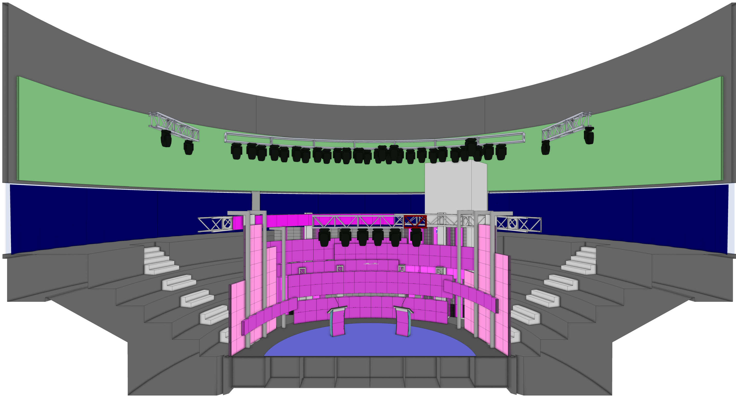
FRONT ELEVATION - SHADED
