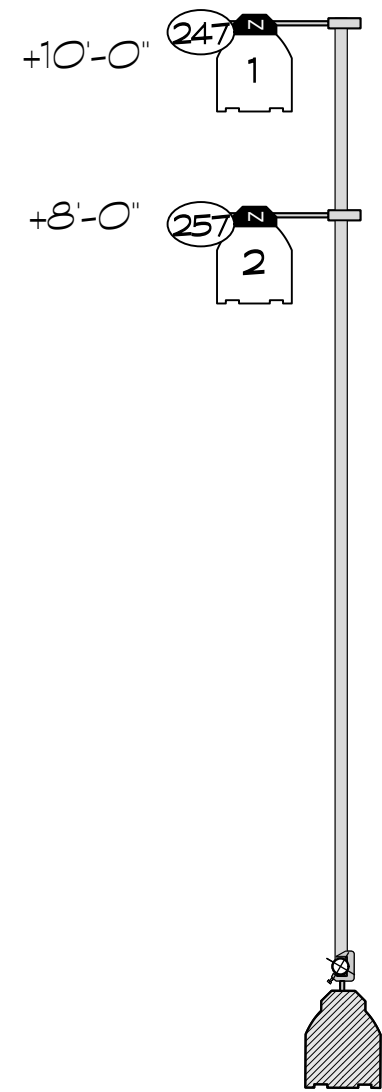
BALCONY BOOM R Note: Position on 2nd floor; see Deck Detail for placement info. Approx Position: +22'-3" @ 3'-6" SR
