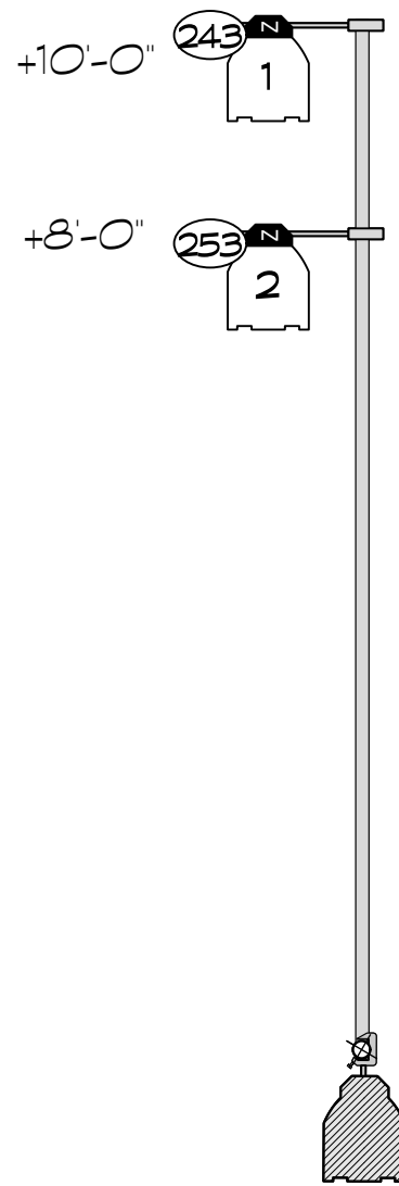
#6 BOOM R Approx Position: +18'-9" @ 5'-0" SR
