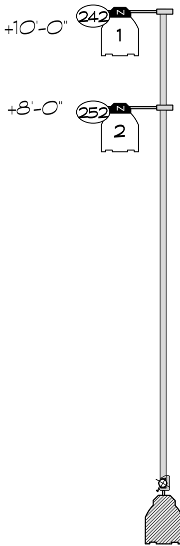
#7 BOOM R Approx Position: +23'-0" @ 2'-6" SR
