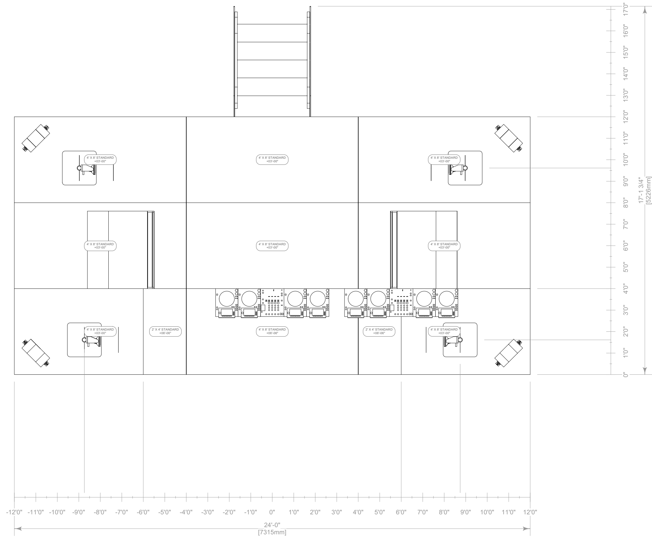
Eric Prydz DJ Booth Detail Top Scale: 3/8" = 1'-0"
