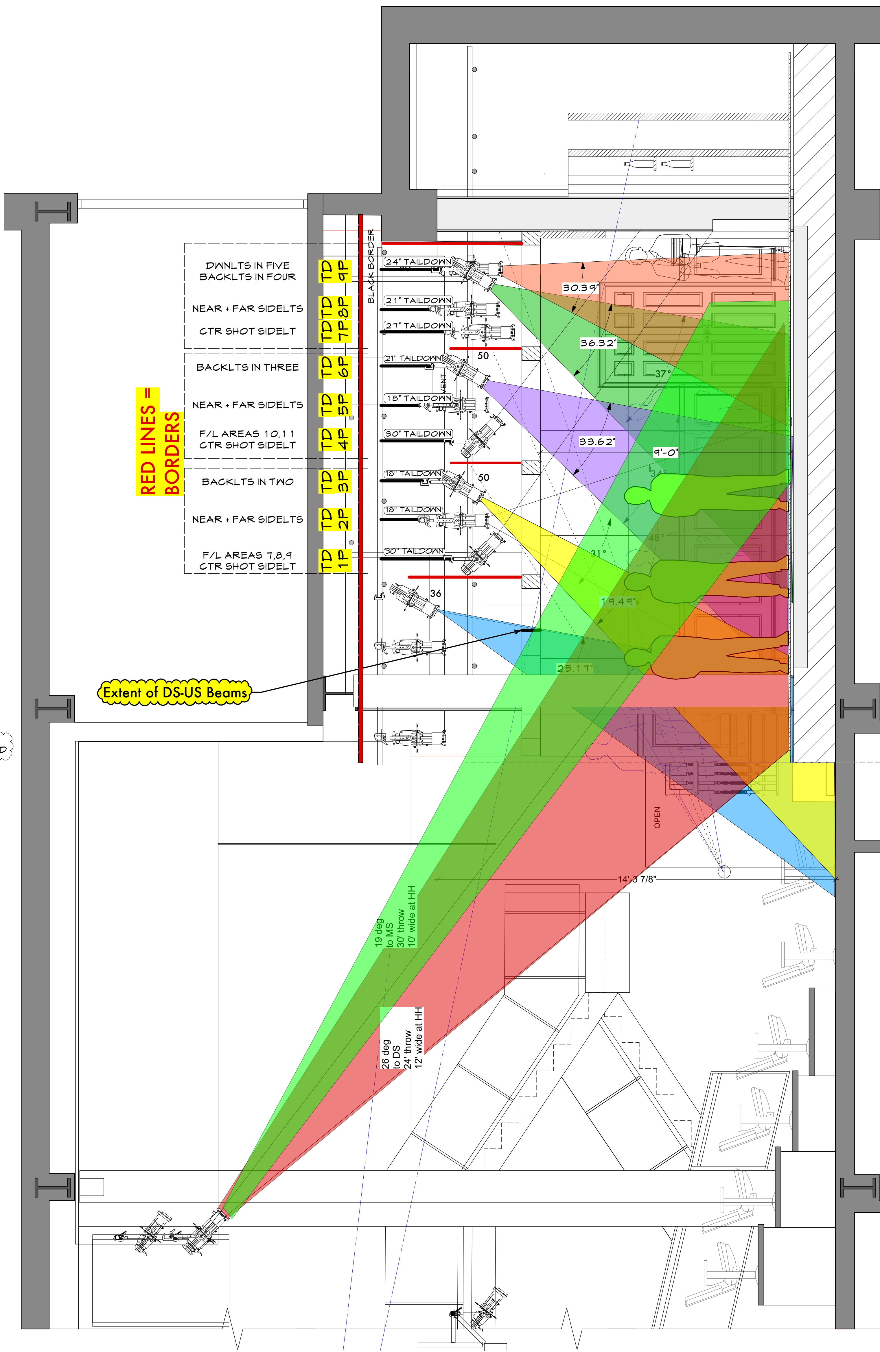
CENTERLINE LIGHTING SECTION TOWARDS S.R.
