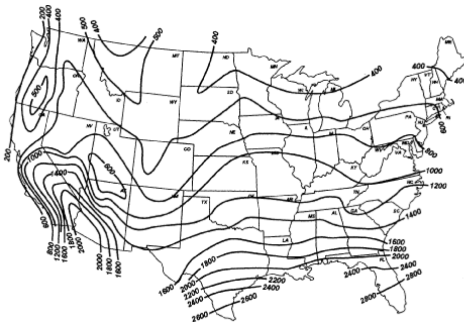
Figure 1—Heating Load Hours (HLH A ) for the United States
