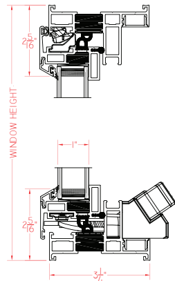
Project-Out Roto
