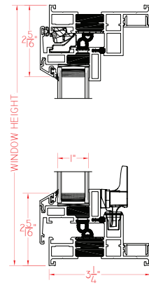
Project-Out Push-Out
