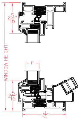
Casement Roto
