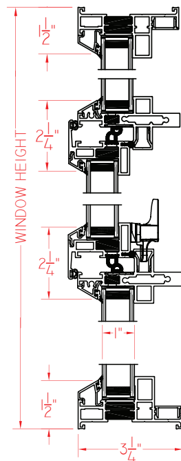
Floating Operator
