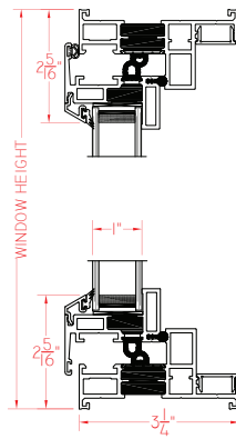
Casement Push-Out
