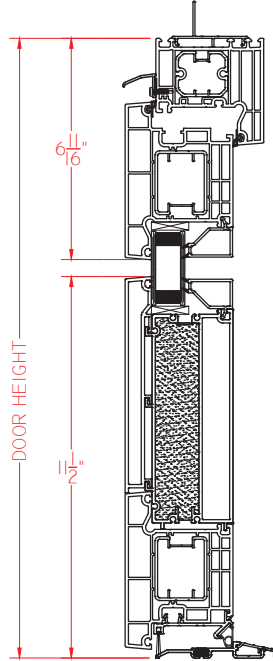
Outswing w/ADA sill
