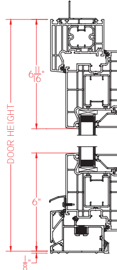
Inswing w/standard sill
