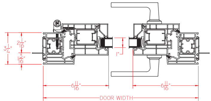
Inswing Models (horizontal cross section)
