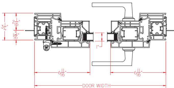
Outswing Models (horizontal cross section)
