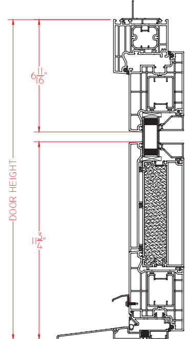
Inswing w/ADA sill
