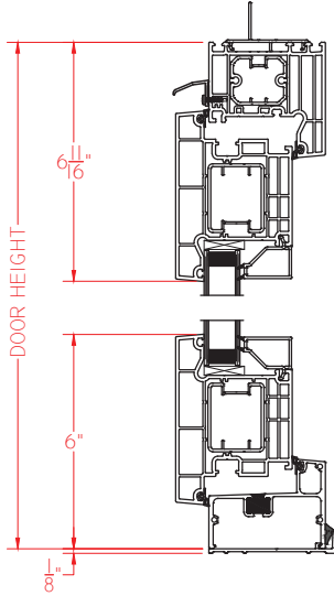
Outswing w/standard sill
