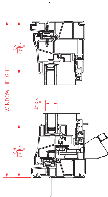
Project-Out (R35) Test size = 48" x 18"
