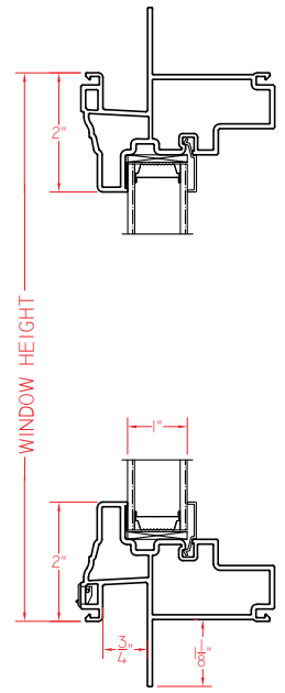
Fixed Narrow (R35) Test size = 60" x 60"
