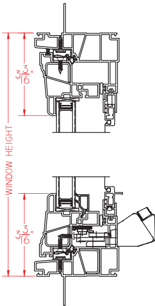
Casement (R35) Test size = 24" x 60"
