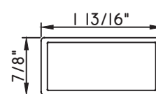
1 3/4"X7/8" M10360 SCALE 1:2
