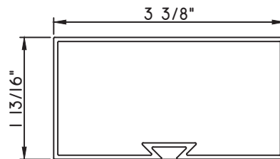
3 3/8"X1 13/16" M23202 (interior side only)
