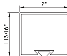
2"X1 13/16" M23199 (interior side only)
