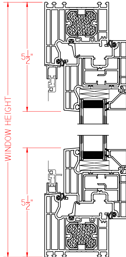
2 VERTICAL CROSS SECTION
