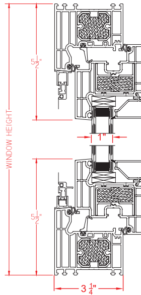
Tilt/Turn
