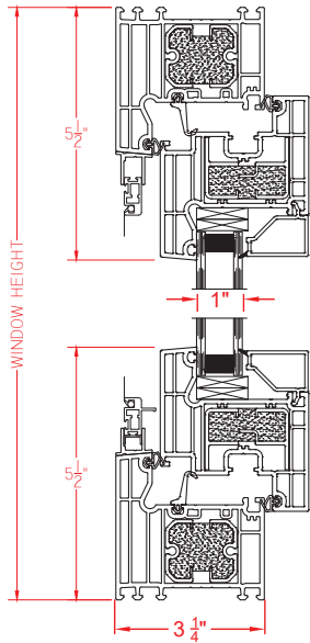
Project-In Casement
