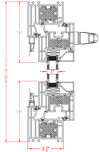
Project-In Hopper
