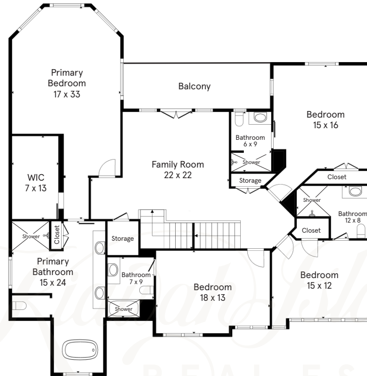
Floor 2
