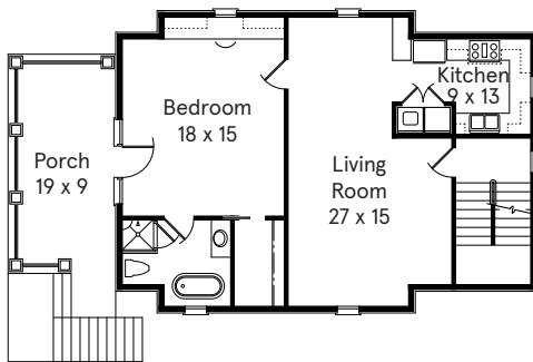
First Floor Guest House
