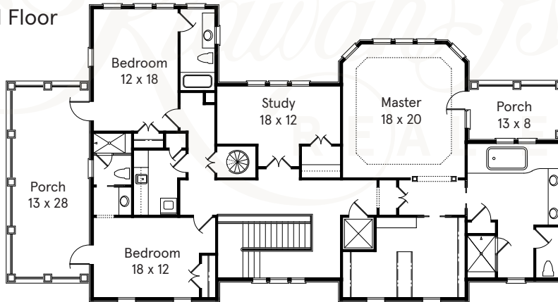
First Floor Guest House
