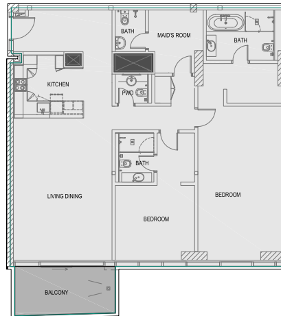
[2] 2-BED L
