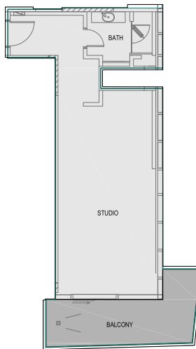
[3] STUDIO S-11.2
