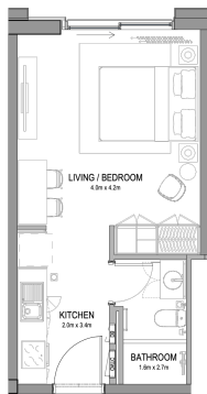
STUDIO - TYPE 1
