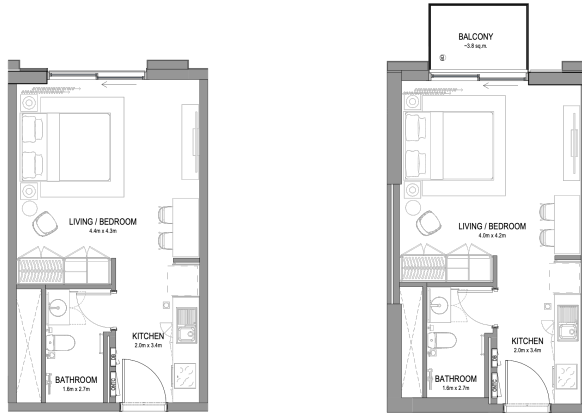
STUDIO - TYPE 3
