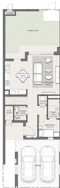
GROUND FLOOR
