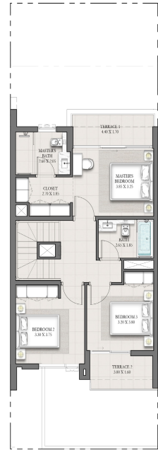
FIRST FLOOR
