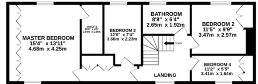
Norcliffe Farm House – First Floor: 743 sq ft (69.0 sq m) approx.
