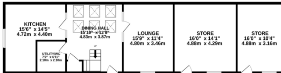
Swallow Barn – Ground Floor: 1012 sq ft (94.0 sq m) approx.
