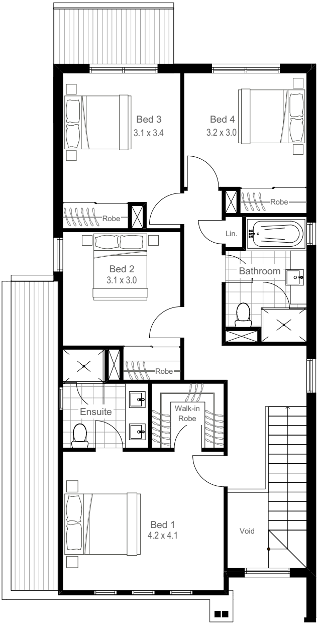
UPPER FLOOR
