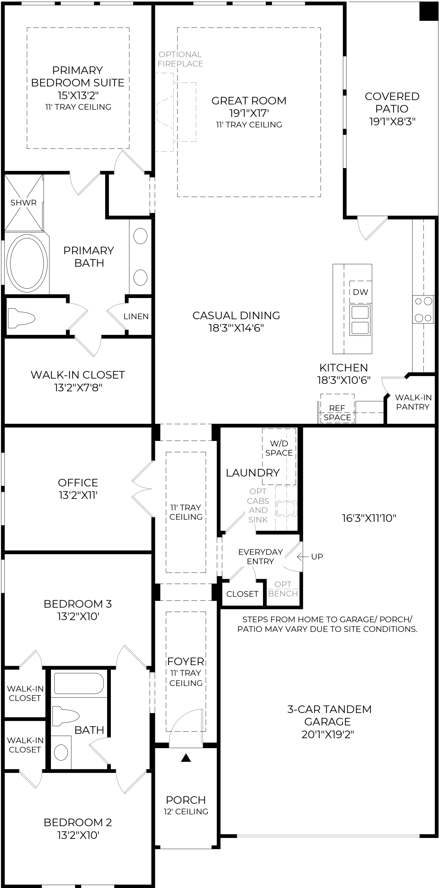
FLOOR PLAN 10' CEILING HEIGHT
