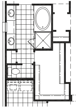
Drop-In Tub with Separate Shower Master Bath Upgrade Option 1300-93
