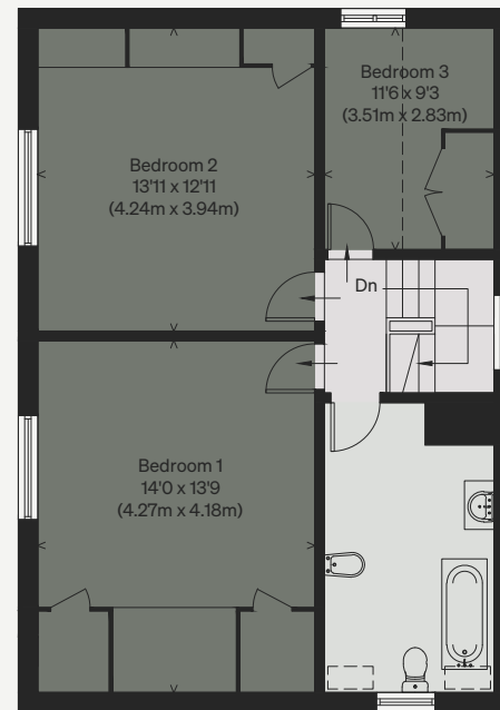
FIRST FLOOR 1
