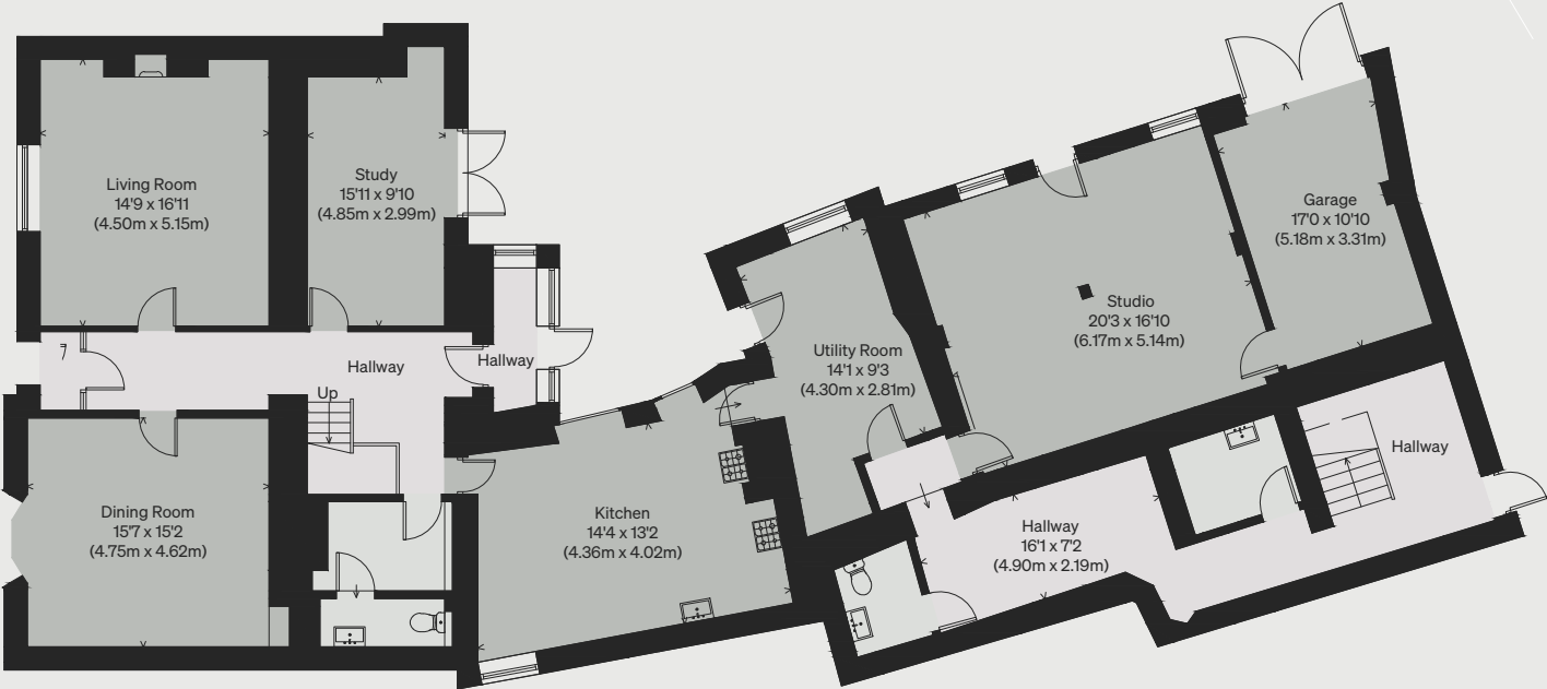
GROUND FLOOR
