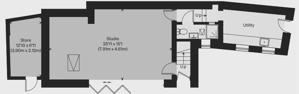
OUTBUILDING GROUND FLOOR
