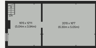
COACH HOUSE - FIRST FLOOR
