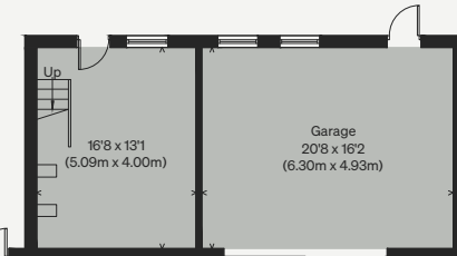
COACH HOUSE - GROUND FLOOR
