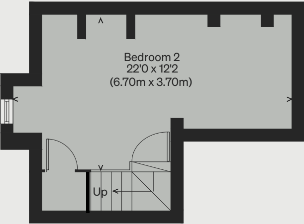
BASEMENT
