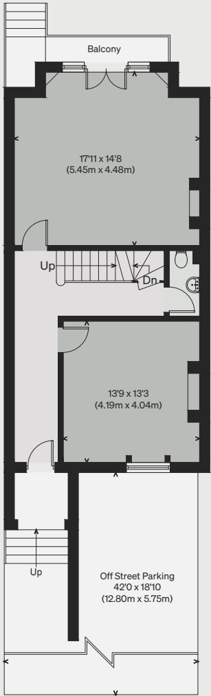
GROUND FLOOR
