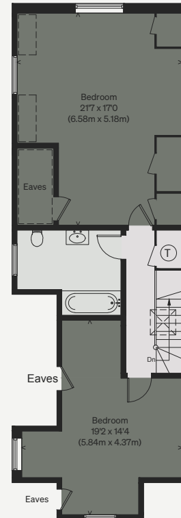
SECOND FLOOR
