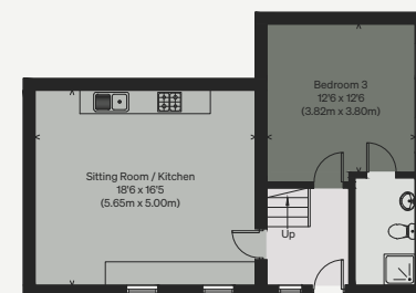
THE OAST GROUND FLOOR
