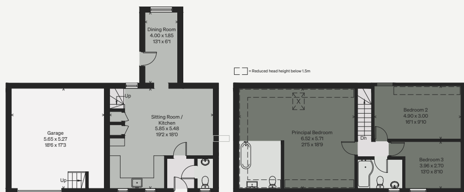
THE COTTAGE GROUND FLOOR
