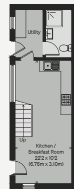
ANNEX - GROUND FLOOR
