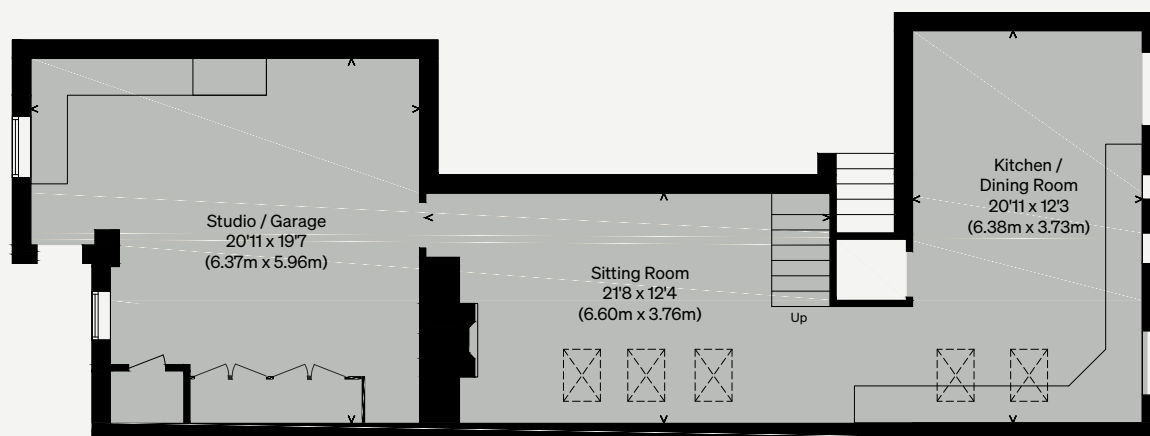
GROUND FLOOR
