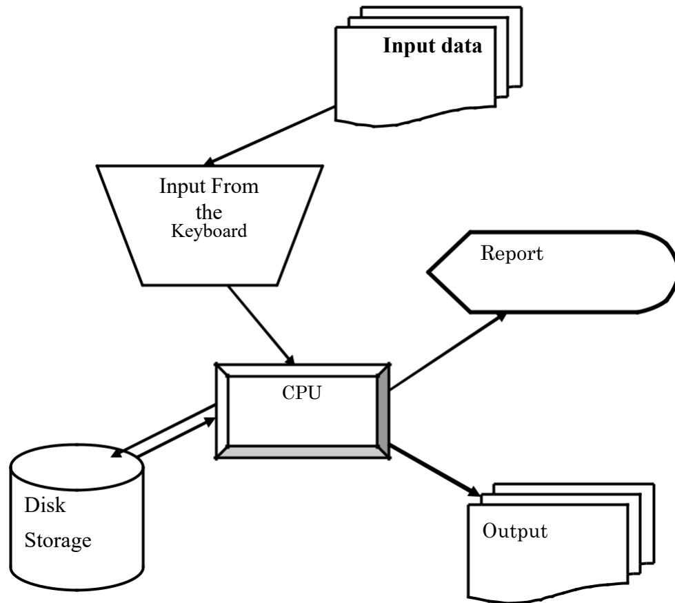
Fig 4.5: System flowcharts.
