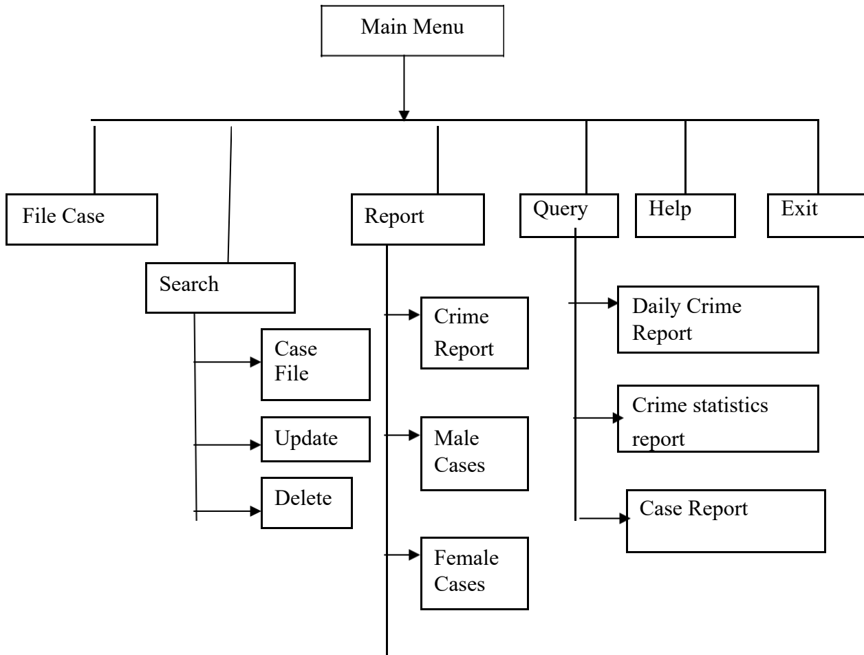
Fig 4.5 Procedure chart.
