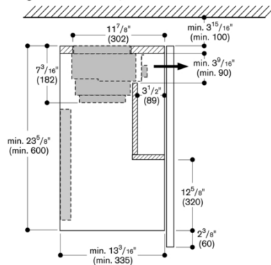
Cross-section top cabinet with AA 211 812 and lowering frame AA 210 490/460
